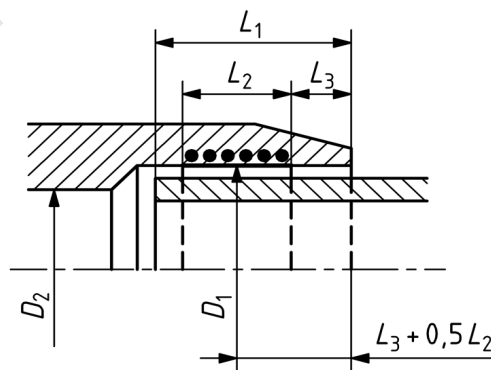
Figure 1 — Dimensions of electrofusion socket fittings
