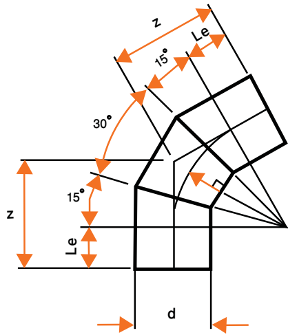
Elbow 60°
