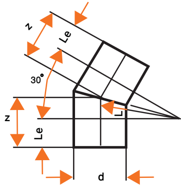
Elbow 30°
