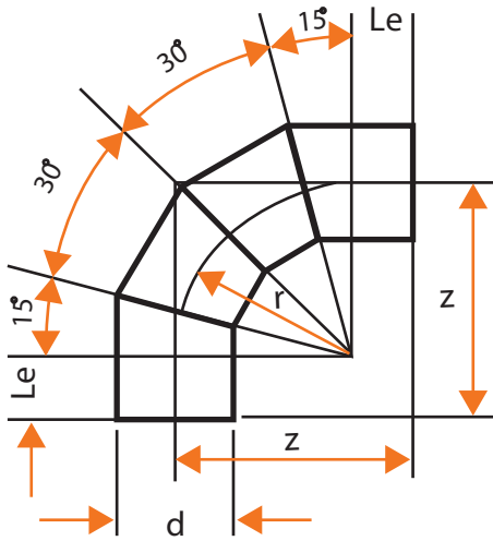
Elbow 90°
