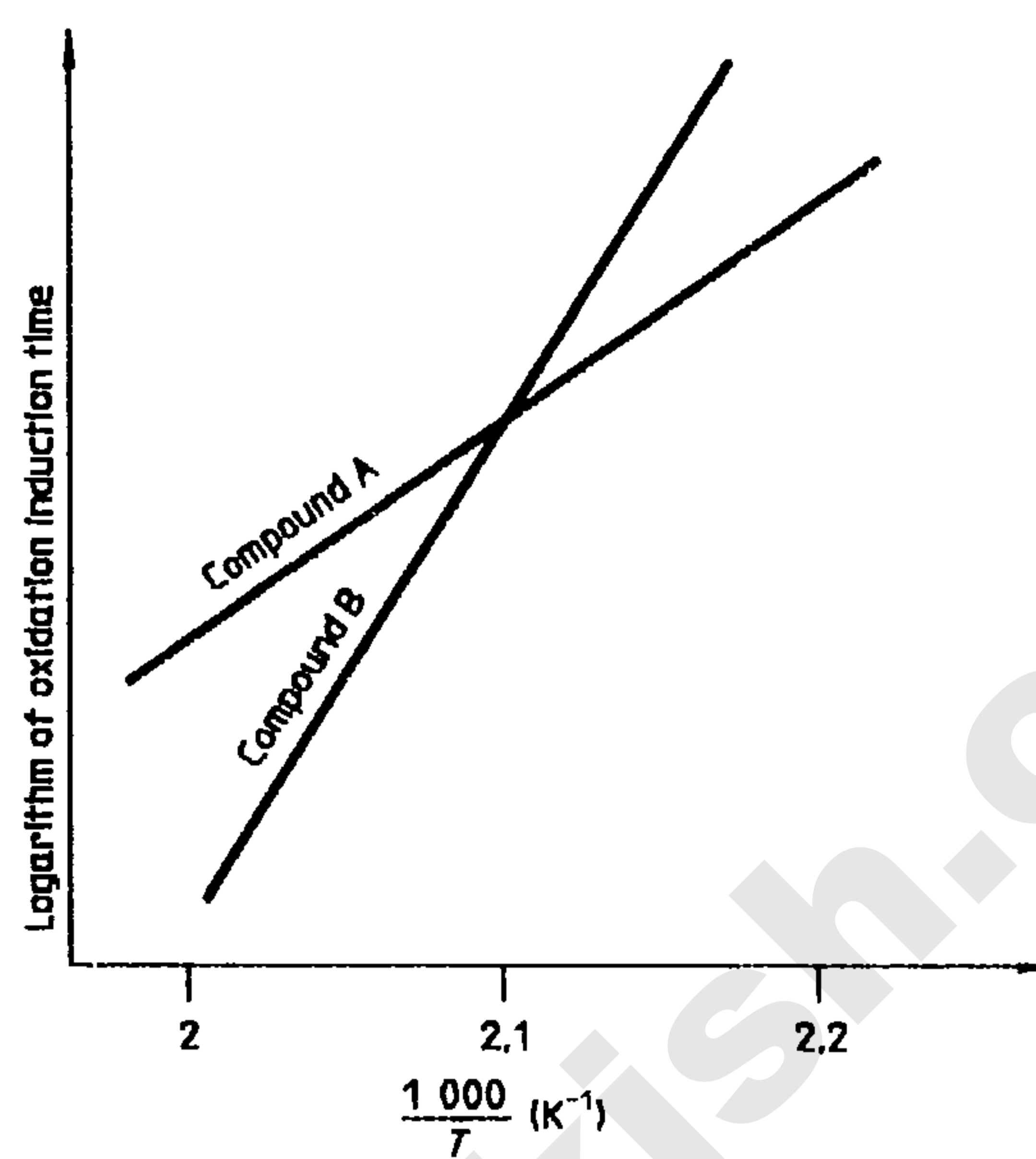
Figure 0.1 — Oxidation of two different stabilizer systems
