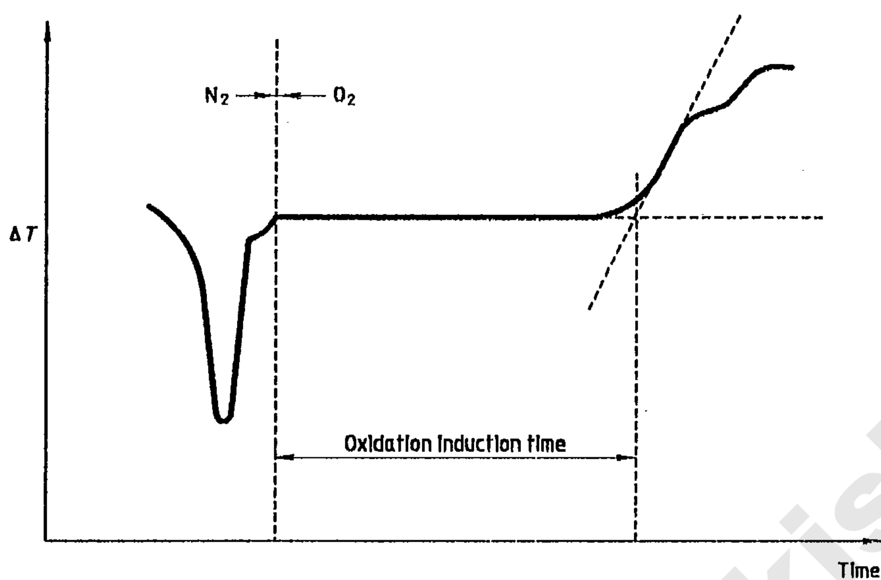
Figure 2 — Typical oxidative thermal stability curve for polyethylene
