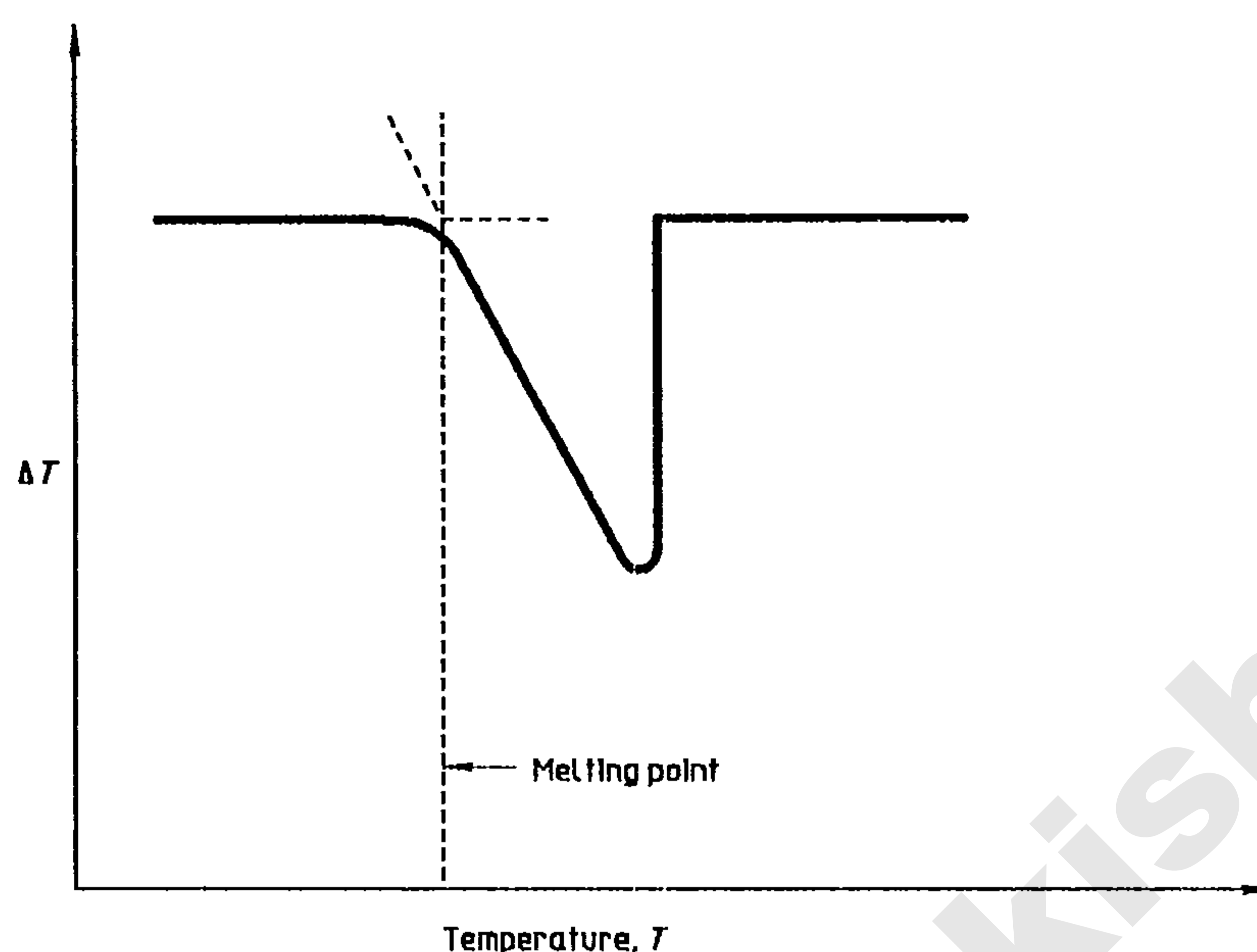
Figure 1 — Typical calibration curve
