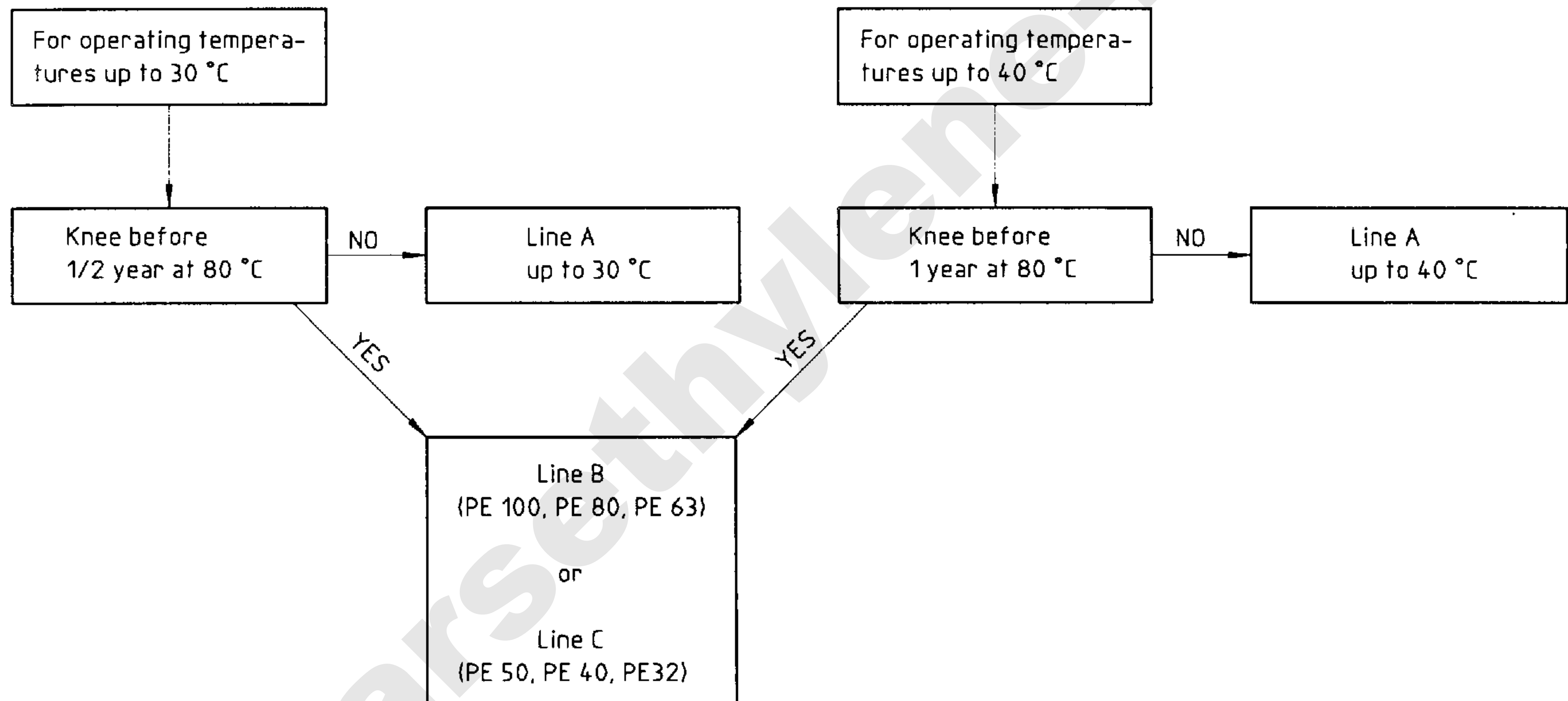
Figure 2 — Determination of reduction line
